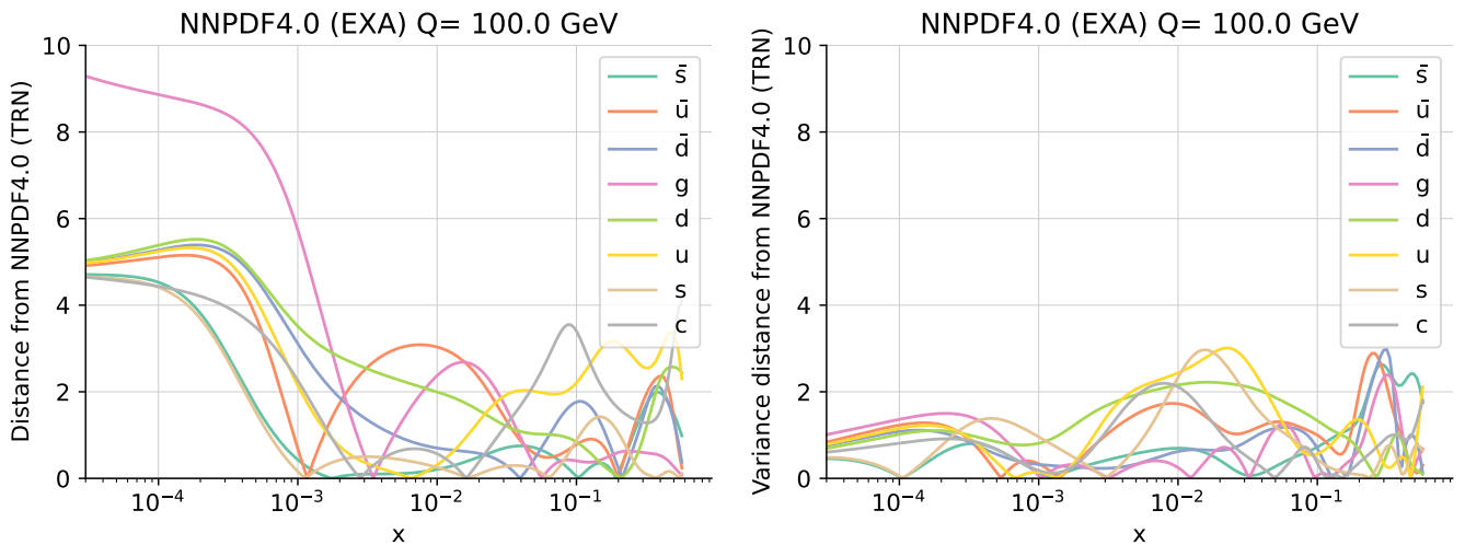
Figure B.1. Statistical distances between the central values (left) and uncertainties (right) of the 100 NNP4.0 PDF replicas whose statistical indicators are compared in Table B.1.
