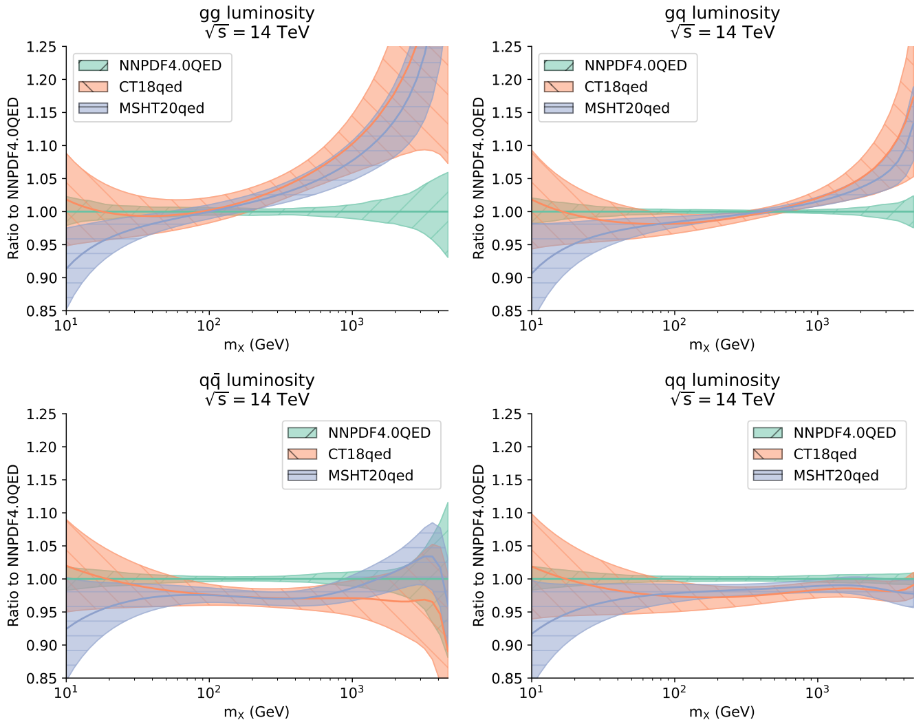
Figure 4.3. Same as Fig. 4.2, now comparing NNPDF4.0QED to MSHT20 [21] and CT18qed [23].
