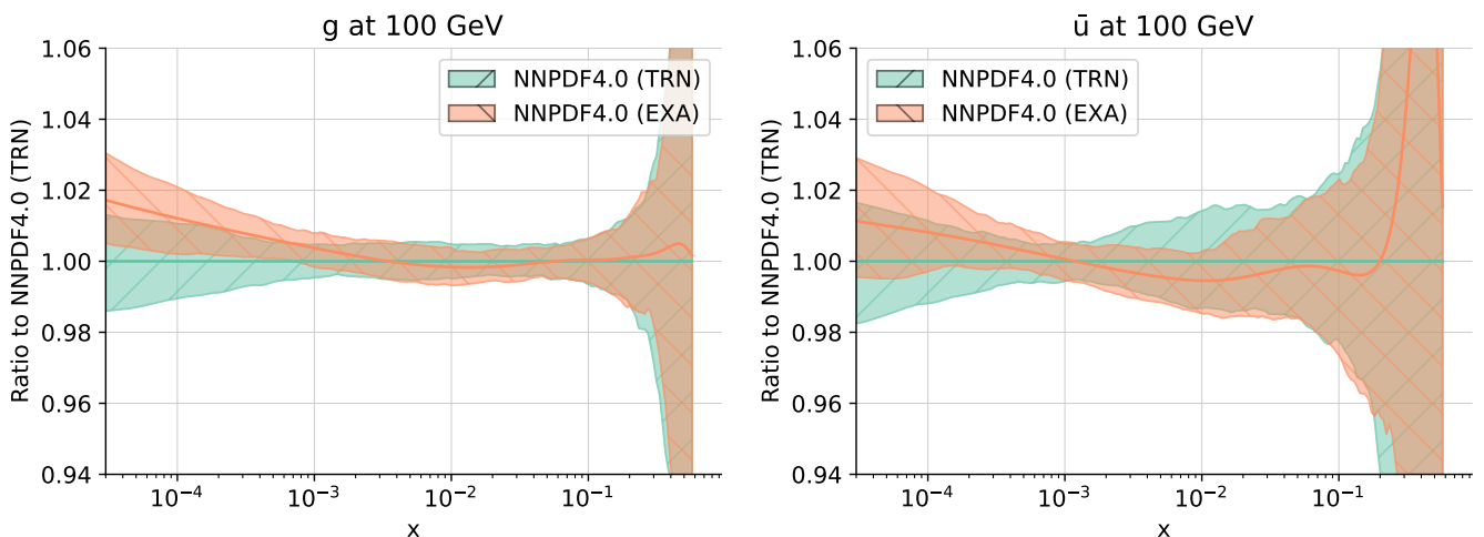
Figure B.2. The gluon (left) and anti-up quark (right) PDFs at Q = 100 GeV from the PDF sets compared in Table B.1 and Fig. B.1. Results are shown normalized to the central value of the PDFs obtained with truncated evolution (published NNP4.0).
