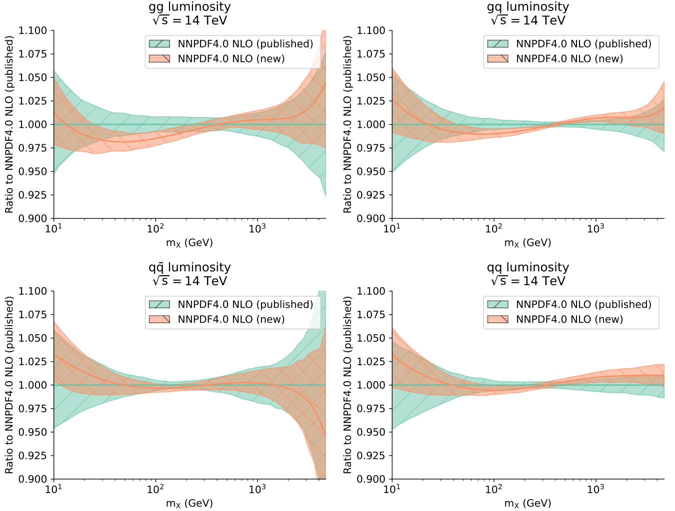
Figure A.4. Same as in Fig. A.2 for the partonic luminosities at the LHC with \sqrt{s} = 14 TeV as a function of the invariant mass m_X . The gg (left) and qg (right) luminosities are shown in the top row, the q\bar{q} (left), and qq (right) luminosities in the bottom row.
